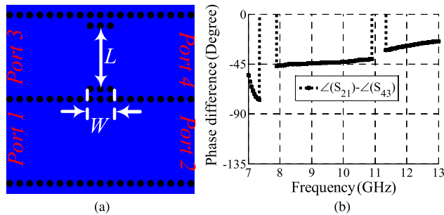
Fig. 3. Configuration and response of 45^\circ phase shifter. a) Configuration of proposed phase shifter, and b) Simulated phase differences. ( W_1 = 5.5 mm, L = 9.4 mm).
