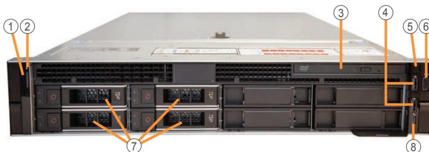
FIGURE 2-3. Deep Discovery Inspector 4200/9200 Front Panel
