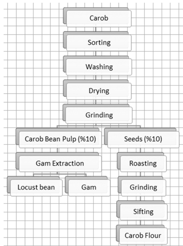
Figure 2. Carob flour production steps
